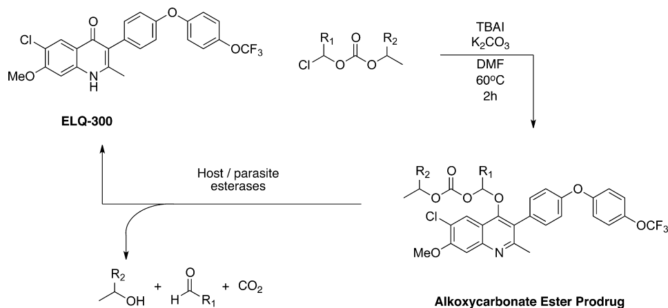
Figure 3. Chemical synthesis and biological cleavage of alkoxycarbonate ester prodrugs of ELQ-300. ELQ-330: R 1 =H, R 2 =CH 3 ; ELQ-331: R 1 =H, R 2 =H; ELQ-387: R 1 =CH 3 , R 2 =H.
