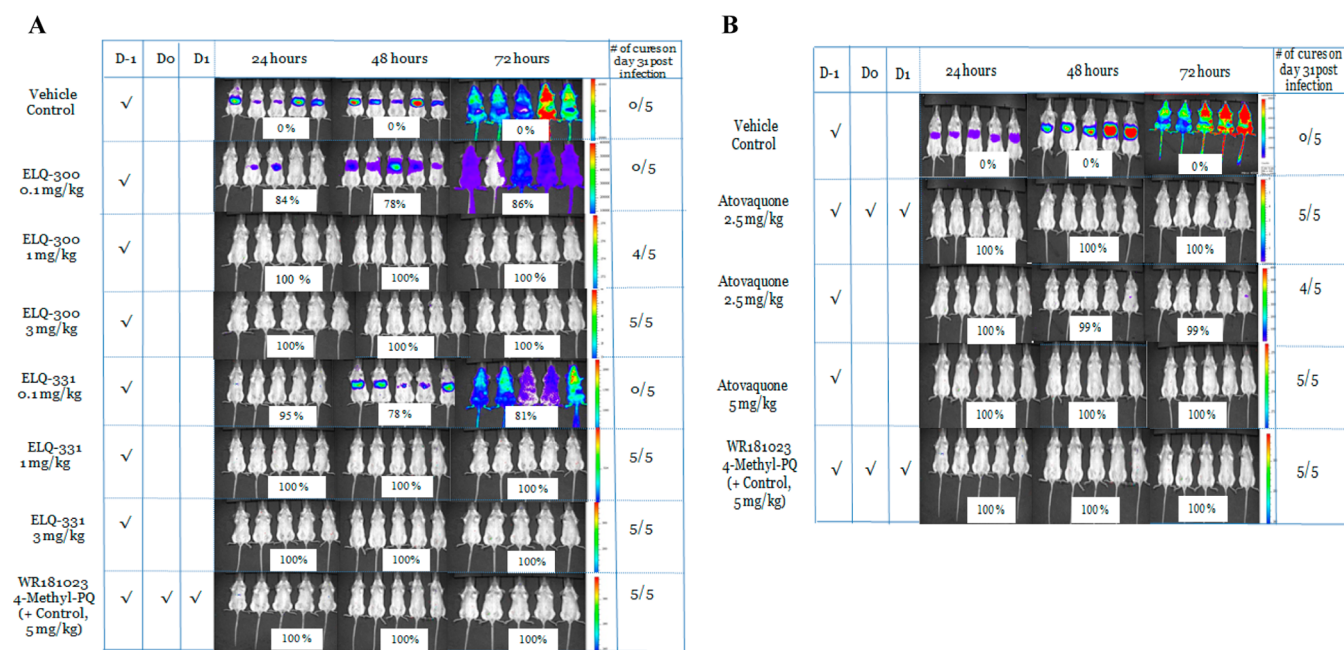
Figure 4. Whole animal bioluminescence imaging of C57BL/6 albino mice infected with 10 000 luciferase-transfected P. berghei sporozoites. Mice ( n = 5 per group) were treated with different doses of ELQ-300, prodrug ELQ-331, or atovaquone according to different dosing regimens: (Panel A) ELQ-300 and ELQ-331 were administered respectively at 0.1, 1, and 3 mg/kg 1 day before sporozoite inoculation; (Panel B) Atovaquone was administered at 2.5 mg/kg on days -1 , 0, and 1 postinfections and at 2.5 and 5 mg/kg on the day before sporozoite inoculation. The bioluminescent signal represents the parasite burden over the body surface area where the red/bright yellow regions represent the most intense signal, followed by green and then blue which represents the weakest signal. A value reflecting the percentage suppression of parasite burden relative to controls at the same time point and based on overall bioluminescence signal appears below in vivo images of each group of animals. ✓: days in which drugs were administered.
