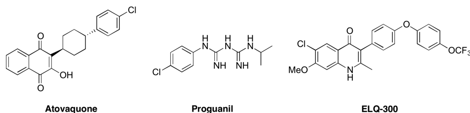
Figure 1. Structures of ELQ-300 and the components of Malarone, atovaquone and proguanil.
